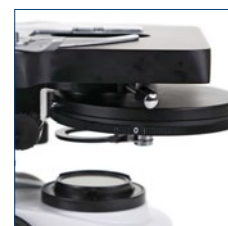
Zernike phase contrast
